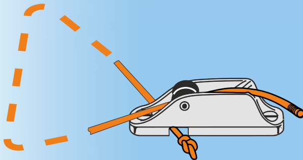
Rigging with a 2:1 advantage
